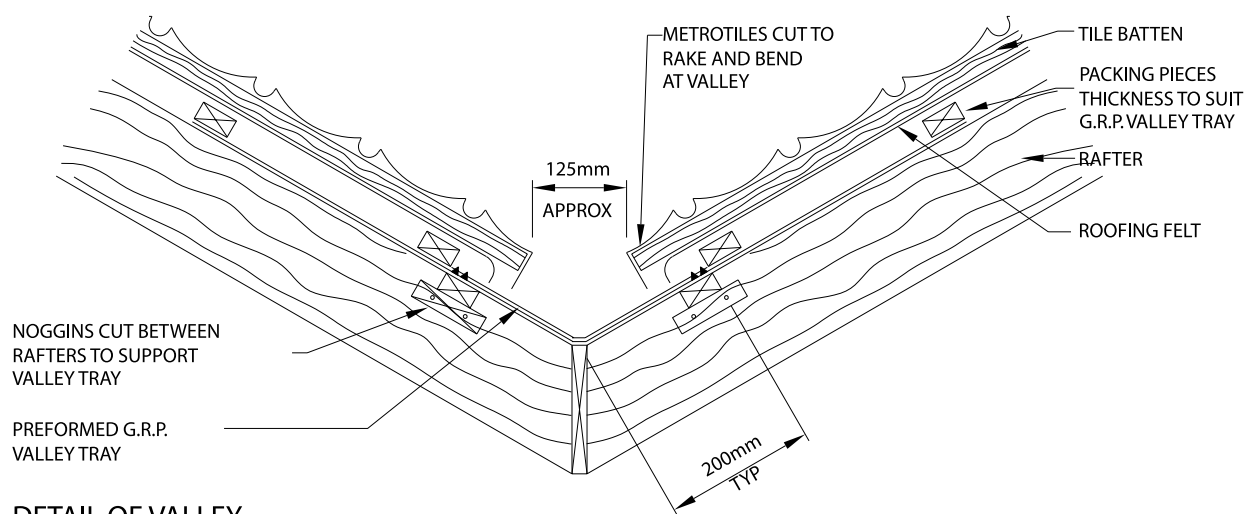
DETAIL OF VALLEY WITH A G.R.P SIMILAR VALLEY TRAY
