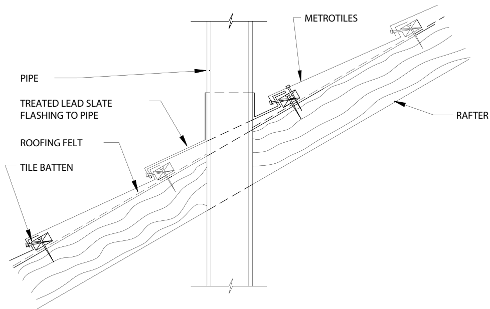
SOIL VENT PIPE THROUGH ROOF
