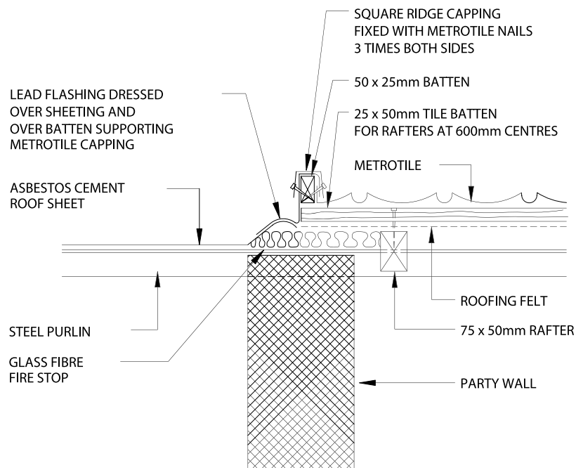
DETAIL OF METROTILE ABUTTING ASBESTOS SHEETS
