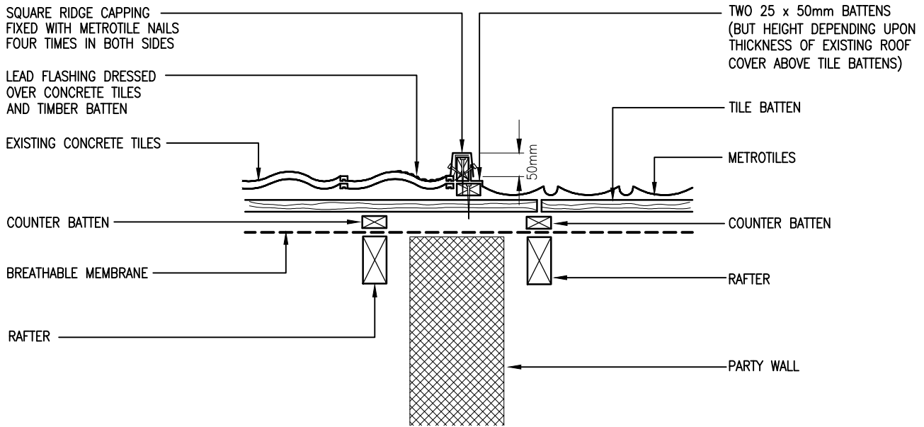
DETAIL OF METROTILES ABUTTING CONCRETE TILES OF PROFILED SECTION
