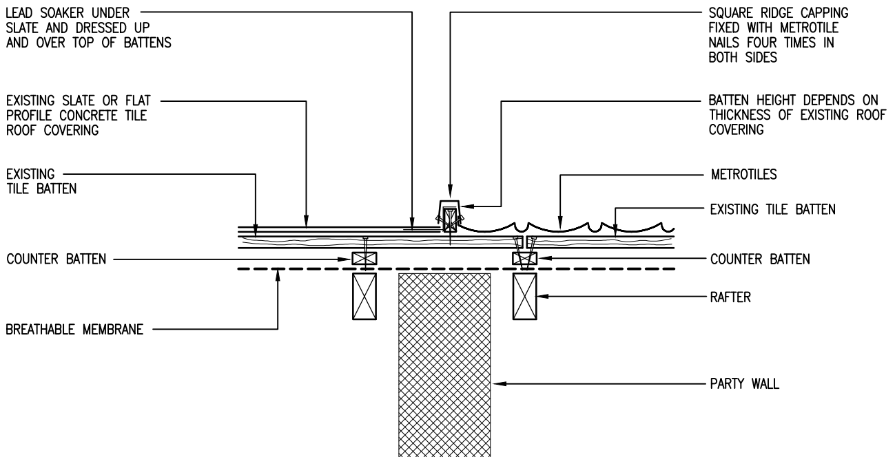
DETAIL OF METROTILES ABUTTING SLATE OR FLAT PROFILE CONCRETE TILE
